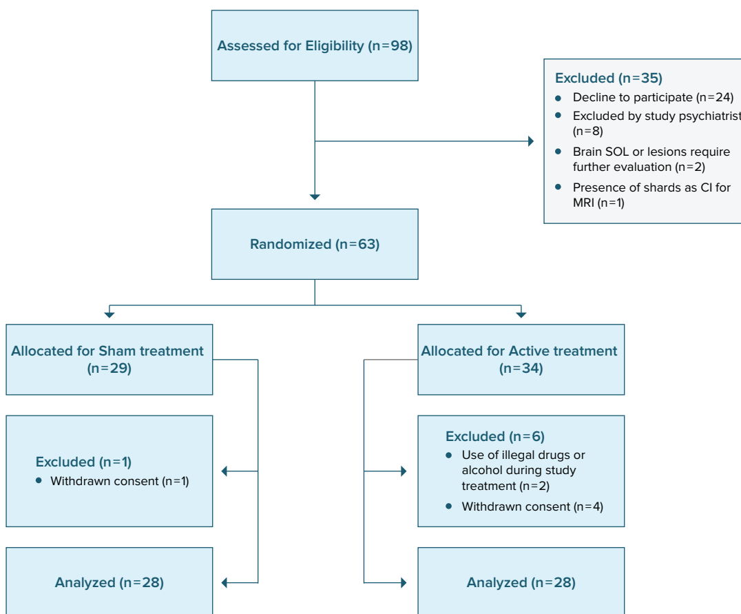
Figure 1. Study Flowchart
